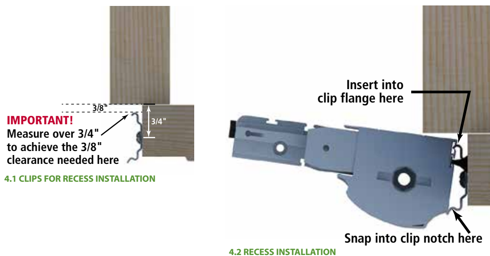
4.2 RECESS INSTALLATION
